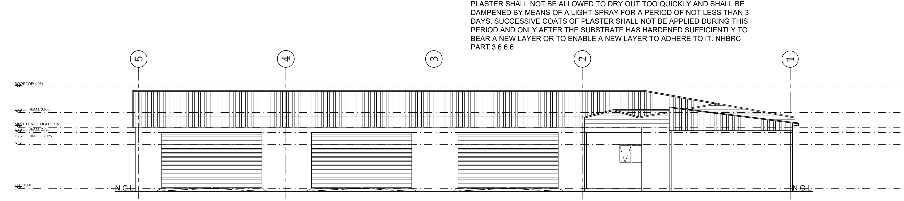
EAST ELEVATION SCALE 1:100
