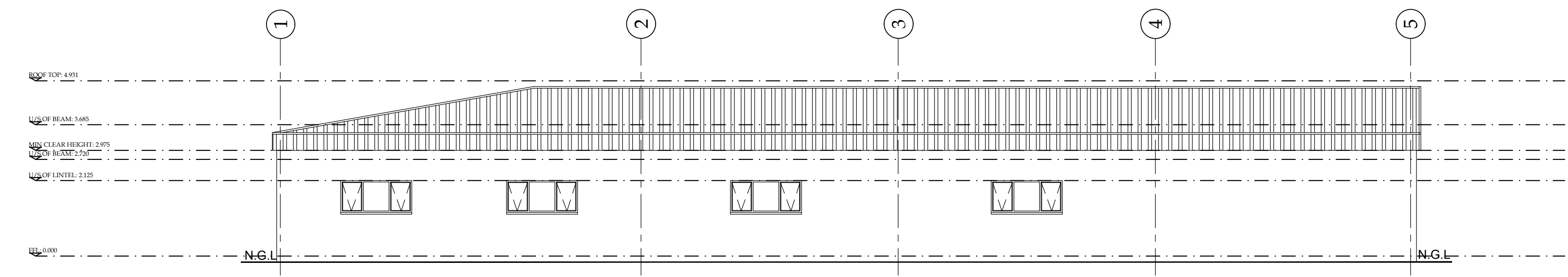
WEST ELEVATION SCALE 1:100
